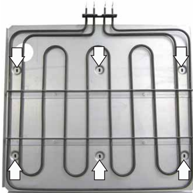
Main Oven Reflector Screw Locations
